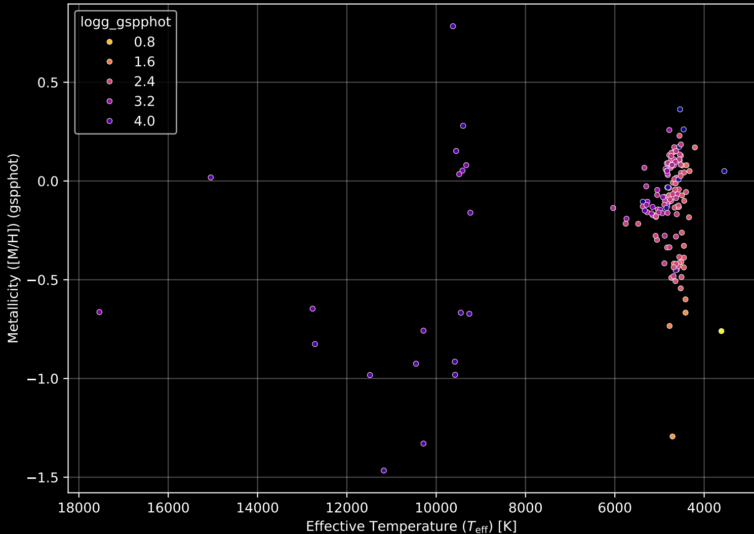
APOGEE DR17 Field: [030+12] Stellar Population Parameters (n= 151)
