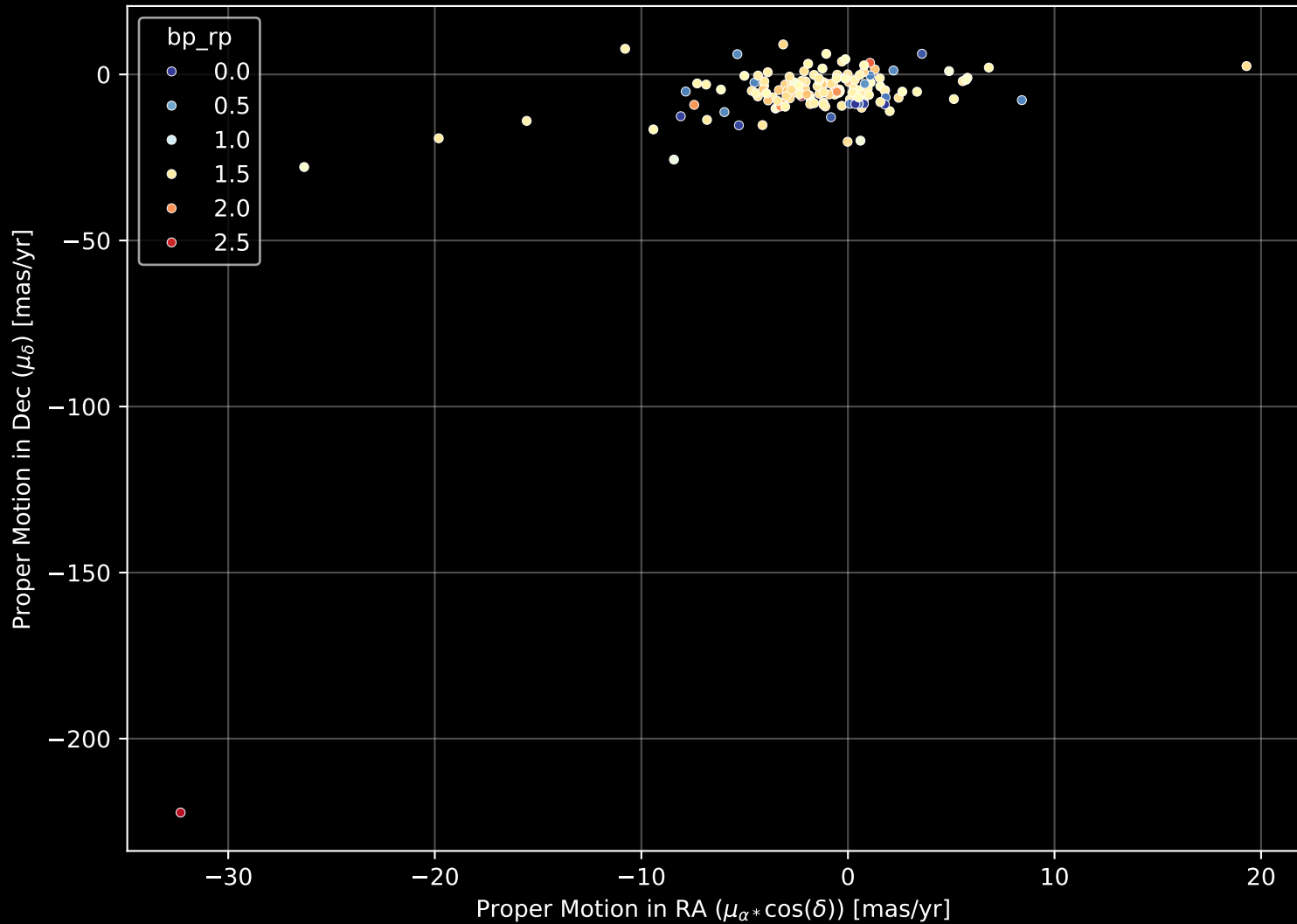
APOGEE DR17 Field: [030+12] Proper Motion Diagram (n= 151)
