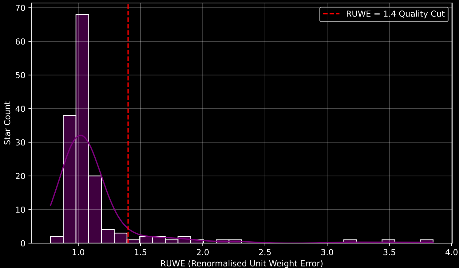
GAPOGEE DR17 Field [030+12] RUWE Distribution (n= 149)
