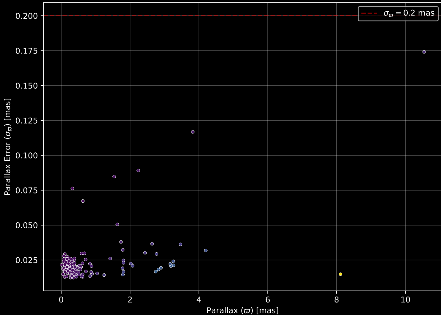
APOGEE DR17 Field: [030+12] Parallax Quality (n= 151)
