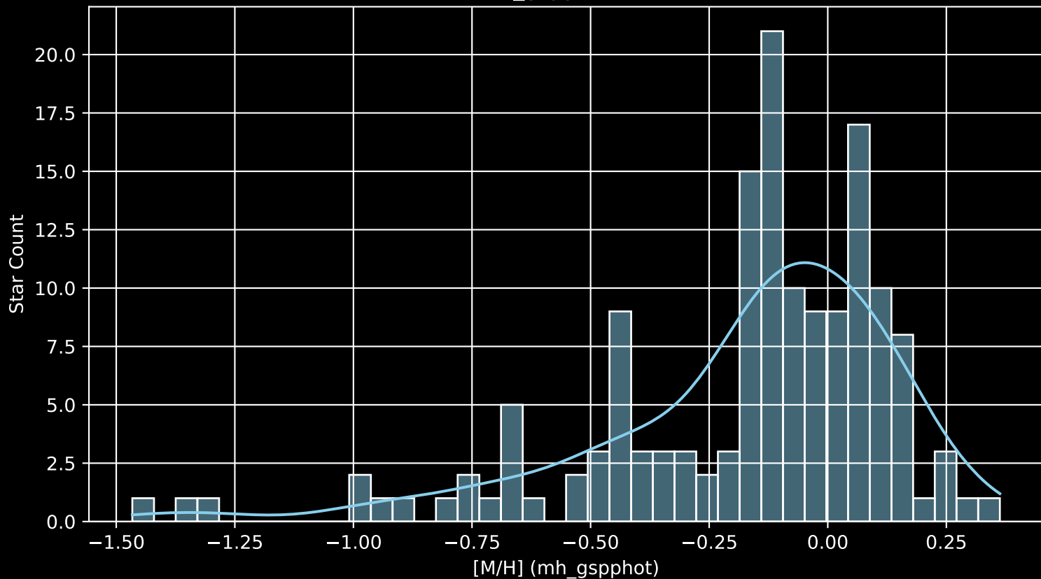
APOGEE DR17 Field: [030+12 [M/H] (mh_gspphot) (n= 150)
