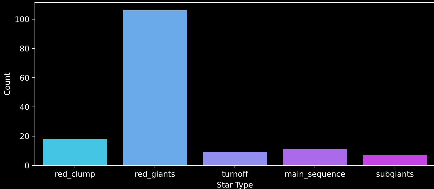
APOGEE DR17 Field: [030+12] Count plot of Star Type
