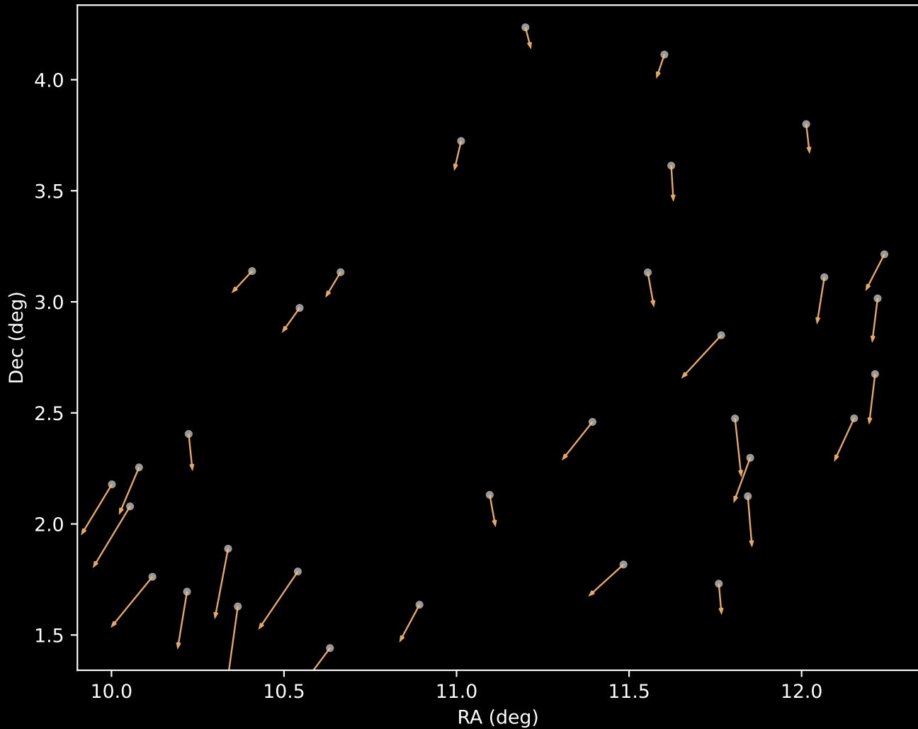
APOGEE DR17 Cluster 3 Proper Motion Vectors (n=33)
