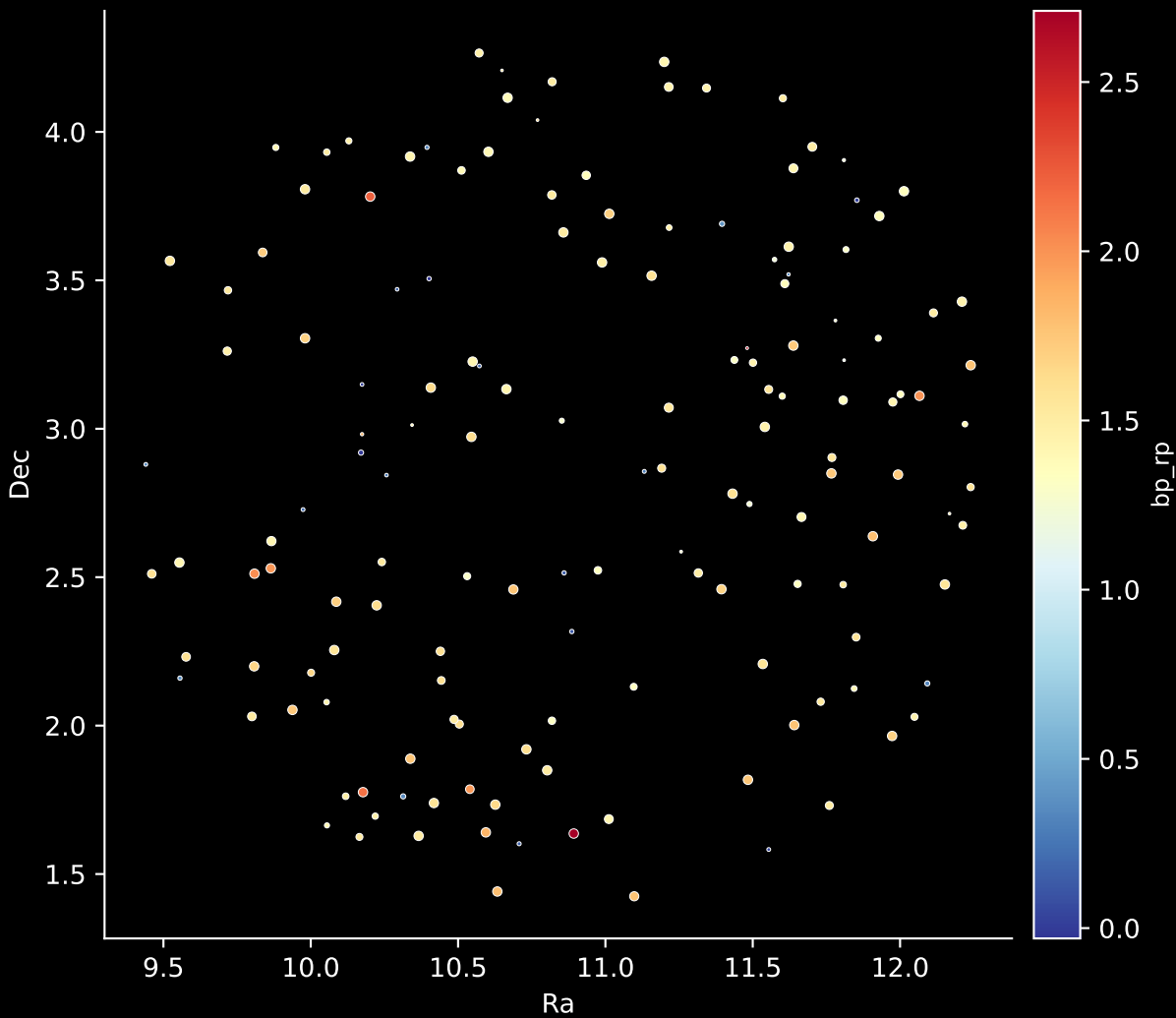
APOGEE DR17 Field: [030+12] Stars: 151
